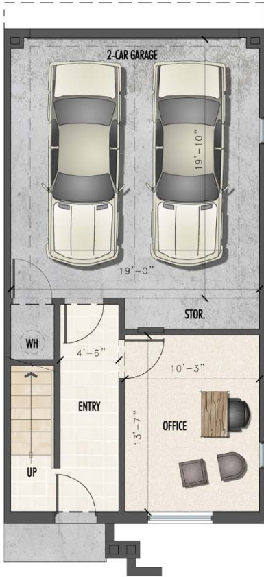
First Level Plan
